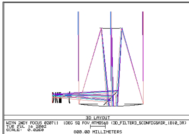
Figure 4. Overall WIYN telescope layout with the one degree corrector shown on the left Nasmyth port.
