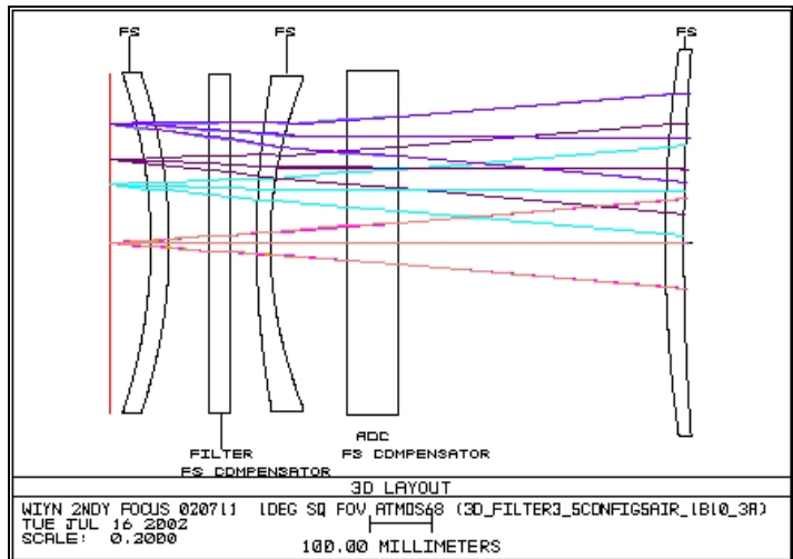
Figure 2. The corrector as above, but now with the ADC replaced by a "dummy" fused silica block to improve the UV transmission.
