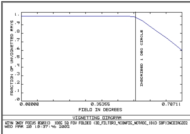
Figure 12. The vignetting function for the one degree corrector as a function of radius. Losses approach 40% in the corners of the field, unless modifications are made to the telescope bearing.
