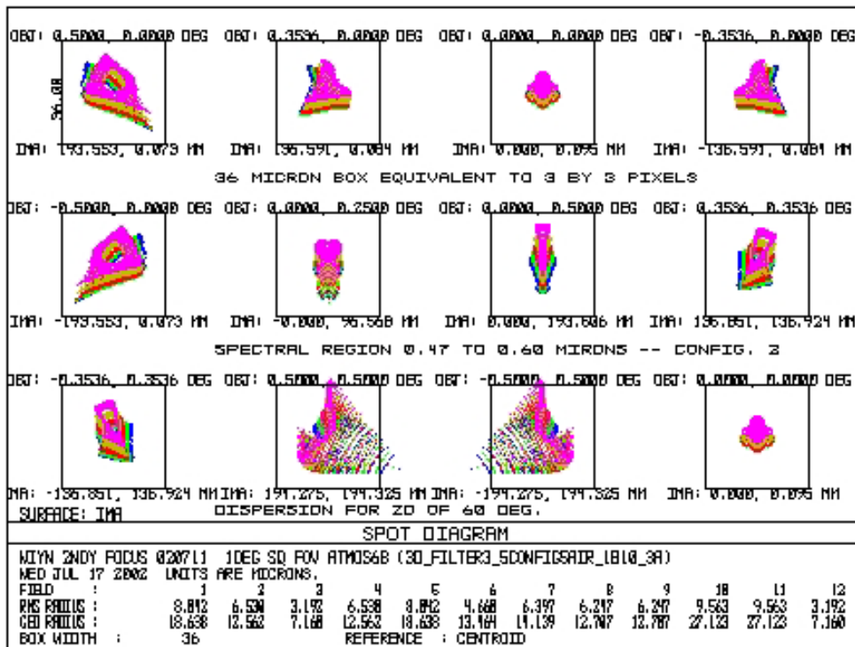
Figure 5. Spot diagrams for the V-band images across the full 1x1 degree field, at zenith distances of 0 (top) and 60 (bottom) degrees. The box sizes for this and the following figures are 3-pixel squares (0.33"x0.33").
