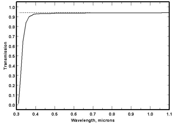
Figure 3. Transmission properties of the entire glass ensemble in the corrector, including losses incurred in the ADC. When the ADC is removed, the transmission is essentially perfectly flat across the spectral range, as shown by the dashed line.
