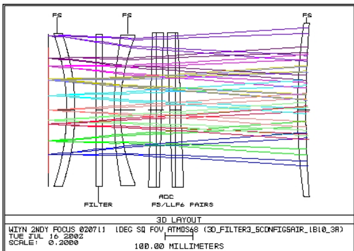
Figure 1. The 1.4 degree FOV corrector for the WIYN 3.5-m telescope with its One Degree Imager. The focal plane is to the left.
