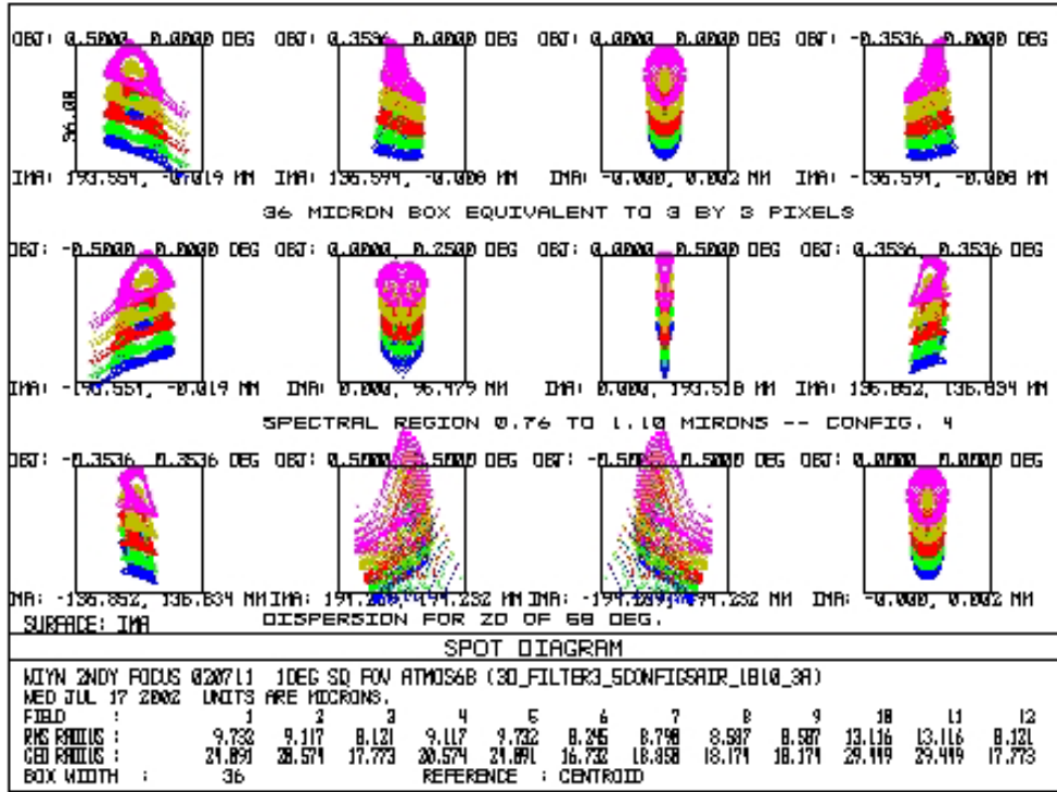
Figure 6. Spot diagrams for the "I"-band images across the field, at zenith distances of 0 (top) and 60 (bottom) degrees.
