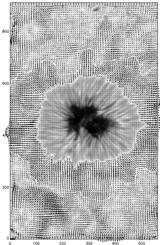
Fig. 4. Map of horizontal velocities of divergence structures, showing large-scale flows. The coordinate unit is 0''.083 (1 pixel). The length of the black bar at coordinates (0, 0) corresponds to 1 \text{ km s}^{-1} . Note that the velocity scaling differs from Fig. 1. The velocities inside the spot were set to zero. The background represents the average image of the white-light series. The moat region is outlined by a white contour.
