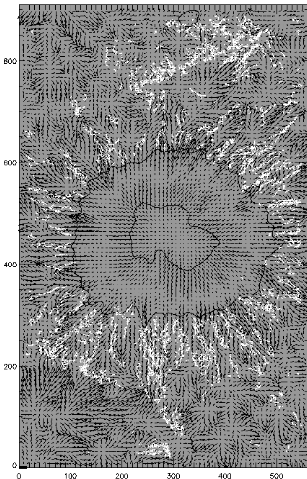
Fig. 7. Positions of GBPs (white) superposed on the map of horizontal velocities (LCT, 2 h averaging).
