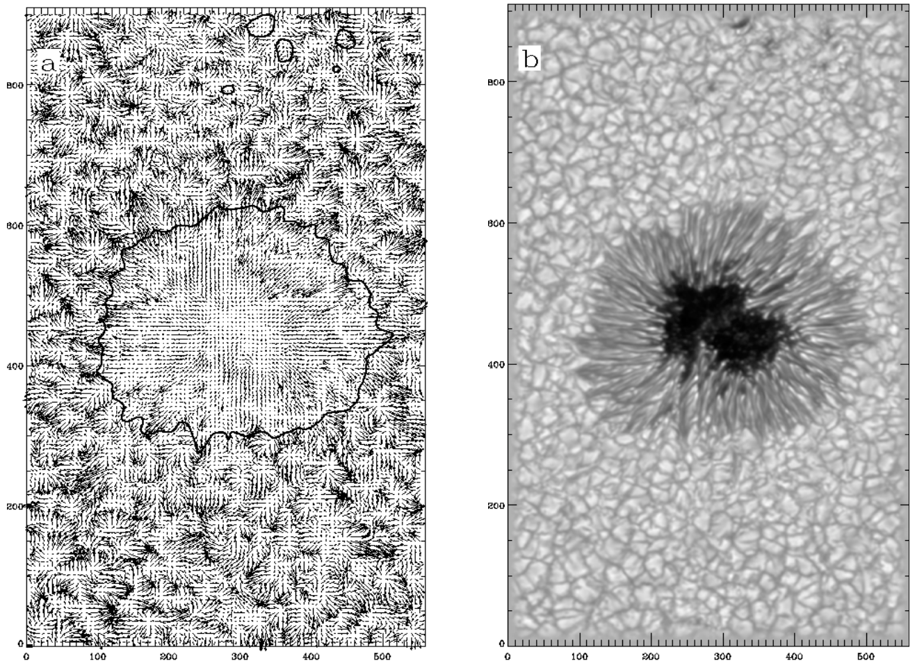
Fig. 3. a) One of the 24 maps of horizontal velocities, averaged over 5 min. The coordinate unit is 0''.083 (1 pixel). The length of the black bar at coordinates (0, 0) corresponds to 1 \text{ km s}^{-1} . b) Average image of the corresponding 5-min white-light series.
