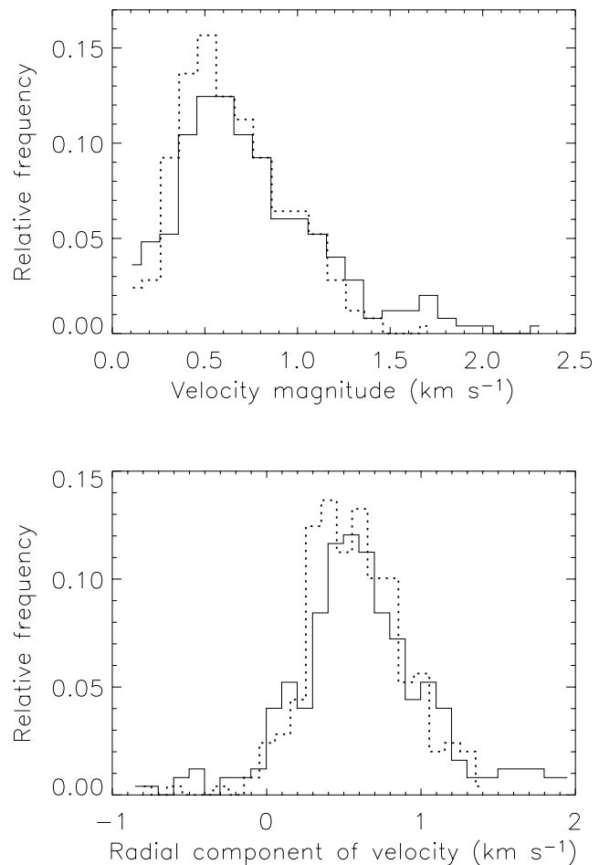
Fig. 8. Histograms of time-averaged velocities of GBPs (solid) and of adjacent granules (dotted) in the moat. Negative radial velocities represent movements toward the sunspot.
