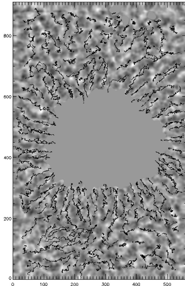
Fig. 6. Trajectories of centroids of the families of granules represented in Fig. 5, superposed on the map of divergence structures (white = positive) averaged over 2 h. The coordinate unit is 0''.083 (1 pixel).
