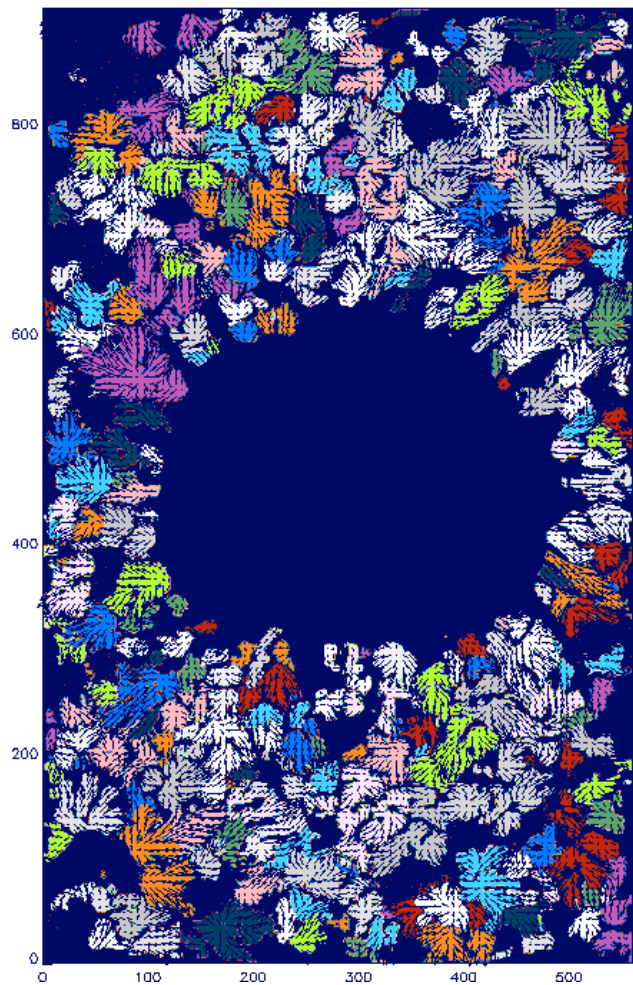
Fig. 5. Areas of families (distinguished by different shades of grey/different colours in the electronic version) superposed on the map of horizontal velocities (LCT, 20-min averaging). The coordinate unit is 0''.083 (1 pixel).
