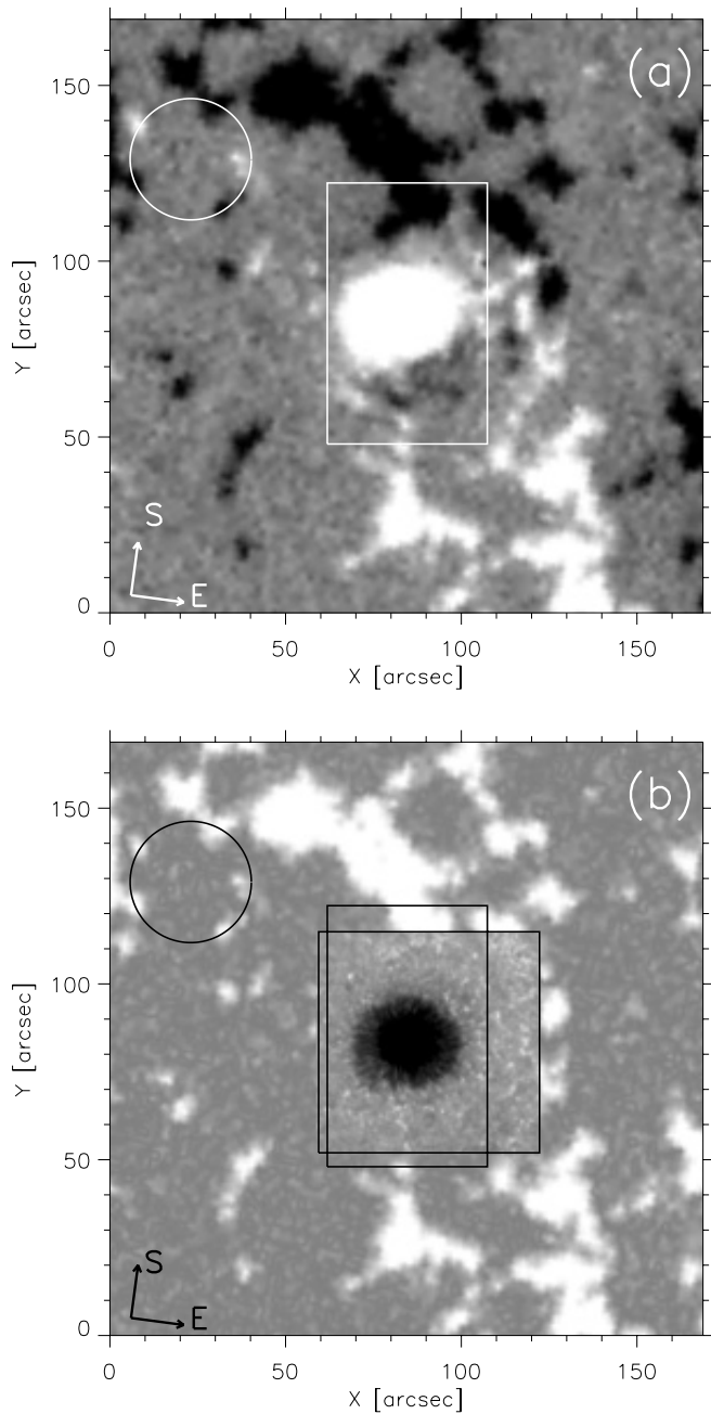
Fig. 2. a) Magnetogram from part of the SOHO/MDI full-disk magnetogram (at 08:00 UT) covering a wide region around the field studied. The signal is saturated at \pm 100 G. b) Ca II K image taken at 07:57 UT (confined by the black square) overlying the magnetic signal in absolute value. The area within the rectangles in panels a) and b) corresponds to the field studied in the white-light and G -band time series throughout this article. The circles in the upper right corners represent a reference size for supergranulation cells ( \sim 35'' ).
