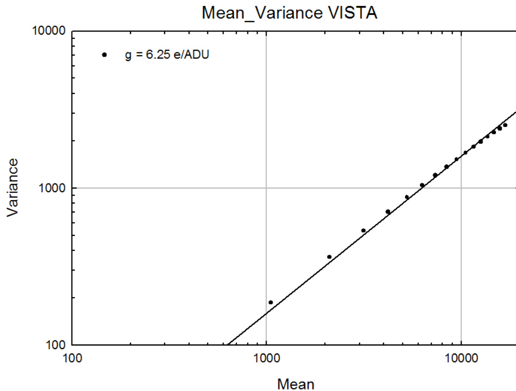
Figure 10: Mean-variance data from Bezawada & Ives for VISTA array SCA-45, plotted on a log-log plot for comparison with the other figures in this report. The line represents a gain of 6.25 e/ADU.
