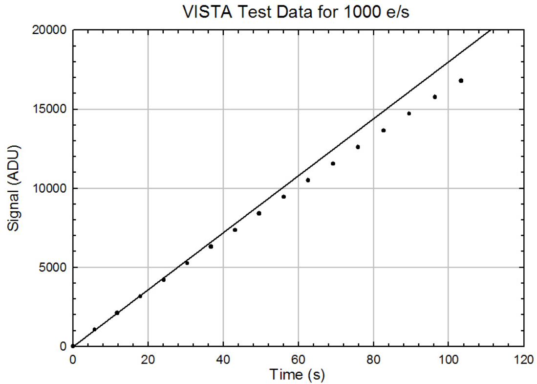
Figure 9: Simulated linearity plot for VISTA array SCA-45 at 1000 e/s using the measured transimpedance conversion gain plot.
