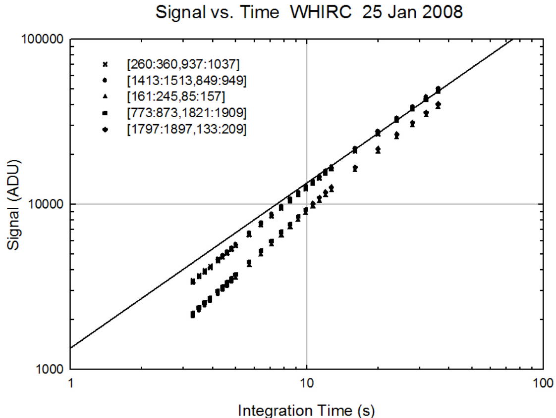
Figure 7: Plot of signal vs. integration time for the data of 25 January 2008. The line represents a slope of 1.0 fit to the data above 20000 ADU.
