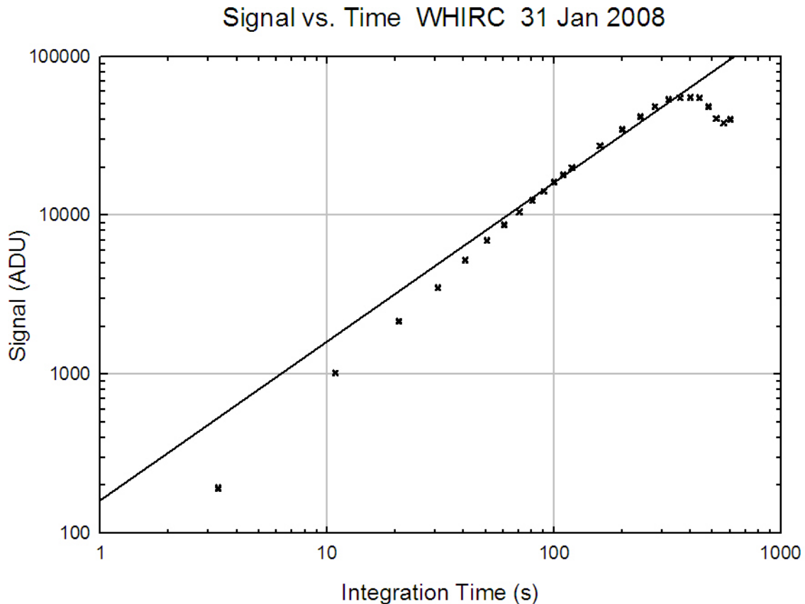
Figure 8: Plot of signal vs. integration time for the data of 31 January 2008. The line represents a slope of 1.0 fit to the data above 20000 ADU. The statistics are for the entire array rather than small subregions.
