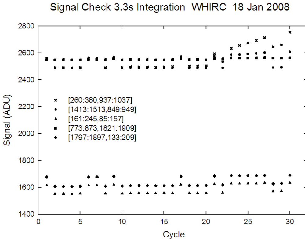
Figure 1: Signal values for five subregions within the “check” frames for the 30 different integration times used in the PTC experiment.
