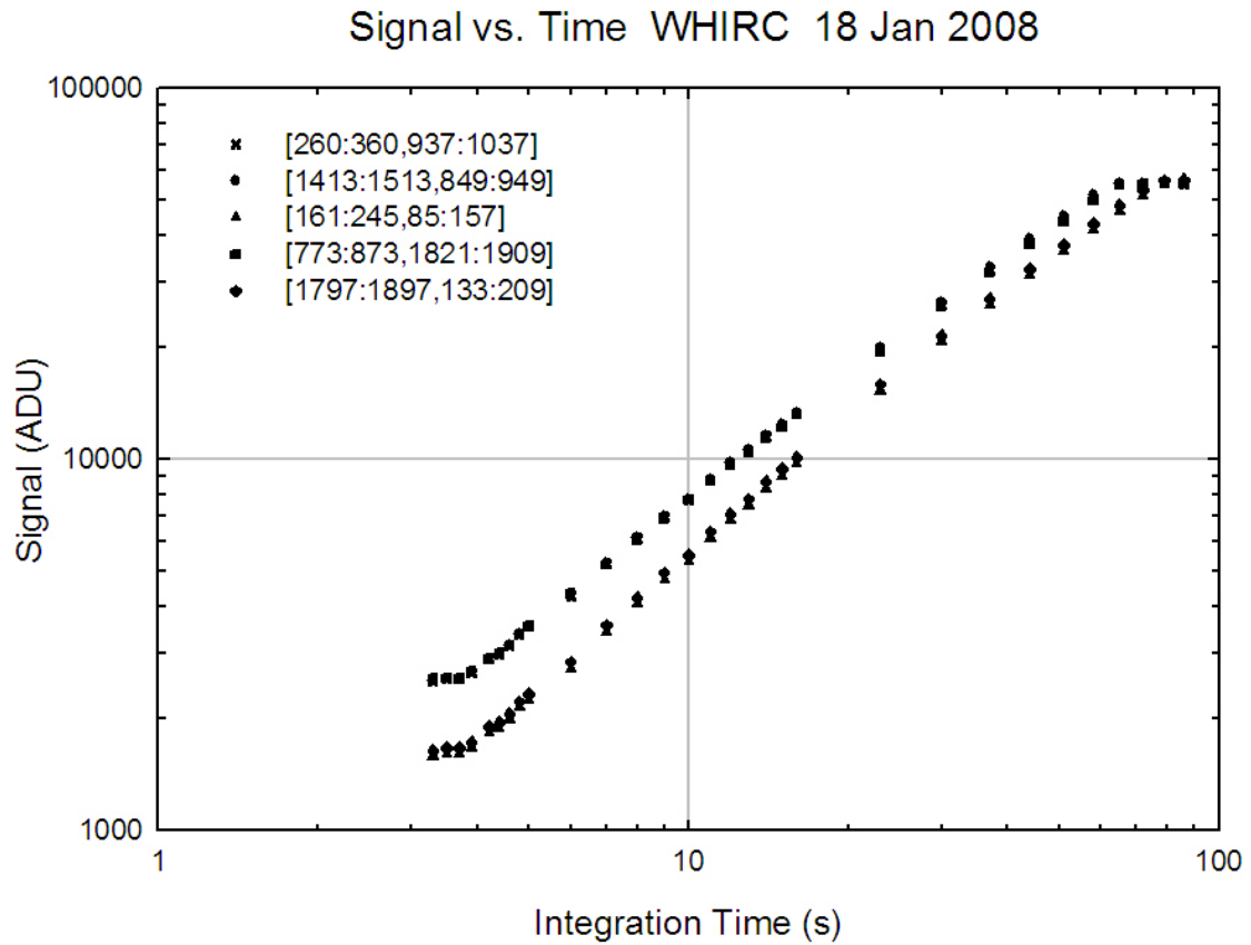
Figure 3: Plot of signal vs integration time for the five subregions used in the mean-variance analysis. The flattening of the curve at short integration times is unexpected.
