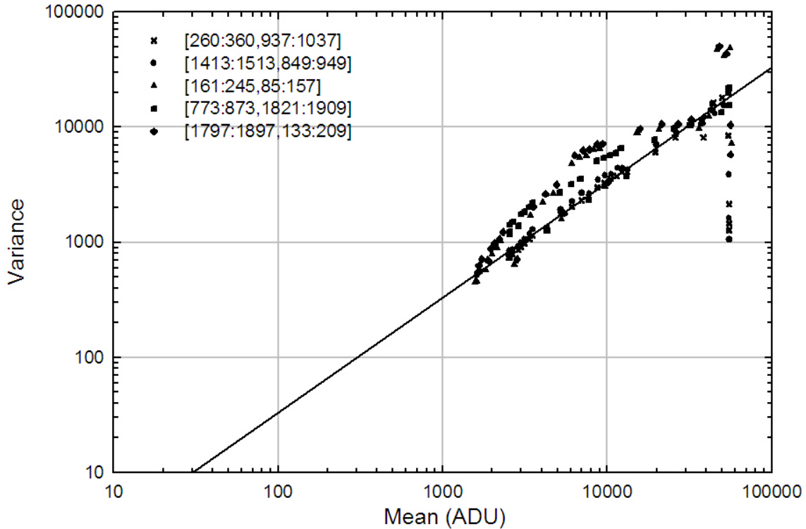
Figure 2: Mean-variance plot for five subregions within the PTC frames. All data were taken at DA4, F1. The read noise from a series of dark frames was 9.6 ADU. The read noise variance of 92 has been subtracted from the variance of the PTC frames. The straight line represents a gain of 3.0.
