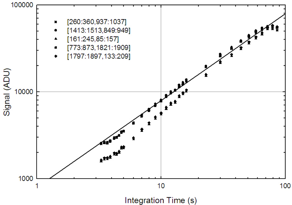
Figure 4: Same as Fig. 3, but with the mean signal values corrected for the estimated variation in flux as determined from the “check” images. The flattening off at short integration times is not as apparent as in Fig. 3, but is still present. The line represents a linear fit (slope=1) through the value for 10 s for the three “high” subregions.
