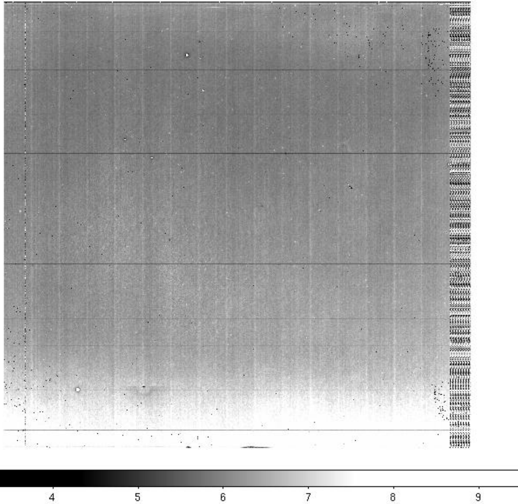
Figure 5: Image of the ratio of the flatfields for 30.0 and 6.0 s. The value in the upper 80% of the array is between 5.5 and 6.4, increasing to near 8.0 at the bottom of the array. The PED artifact [641:285] is weakly visible.
