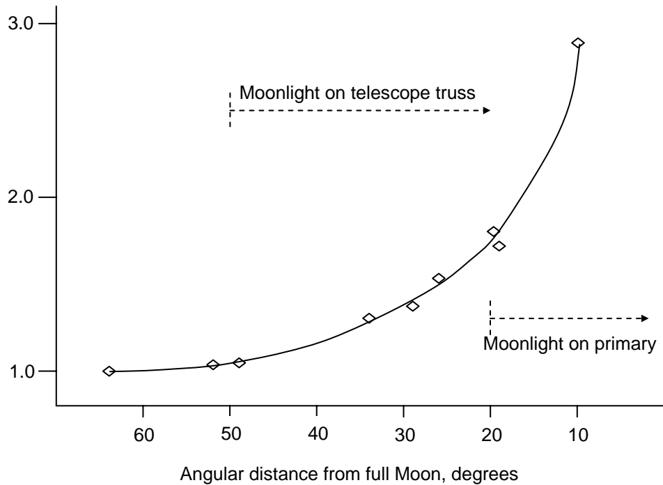
Figure 2. Relative increase in J sky background with proximity to full Moon
