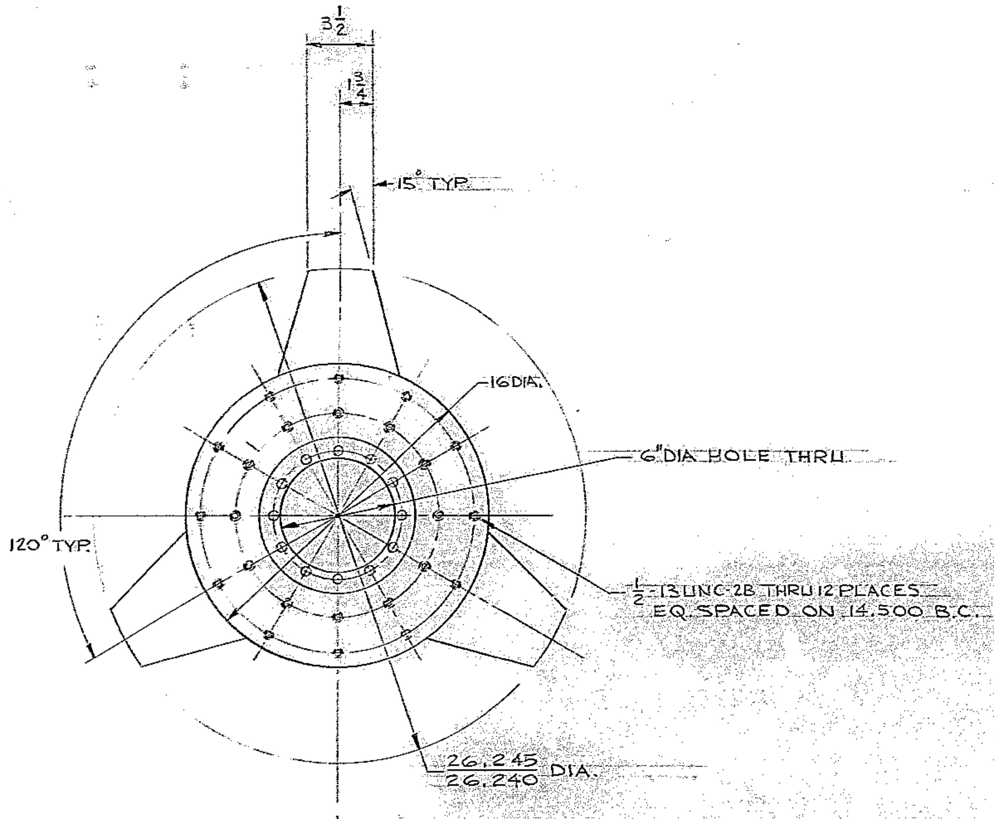
VIEW A-A SCALE 1/4
