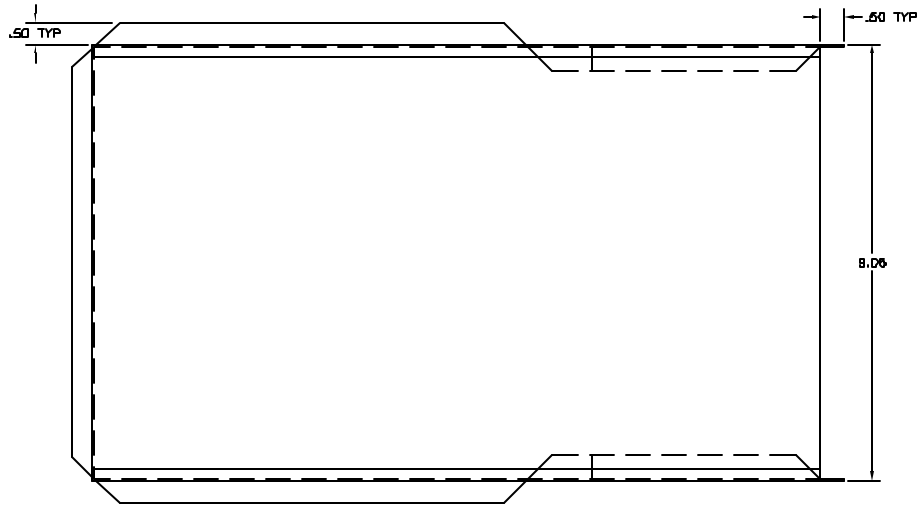
③ ELBOW MATU 32 GA (.0308) GALVANIZED STEEL SHEET FULL SIZE
