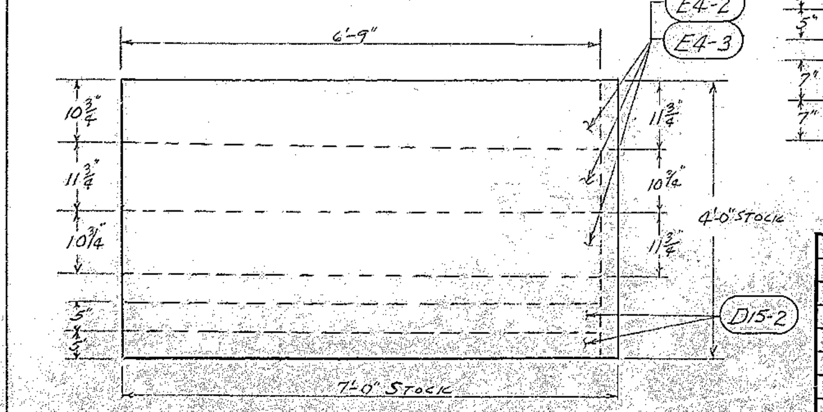
CUTTING LAYOUT SHEET B 6 REQ'D - 3/4" x 1'-0"
