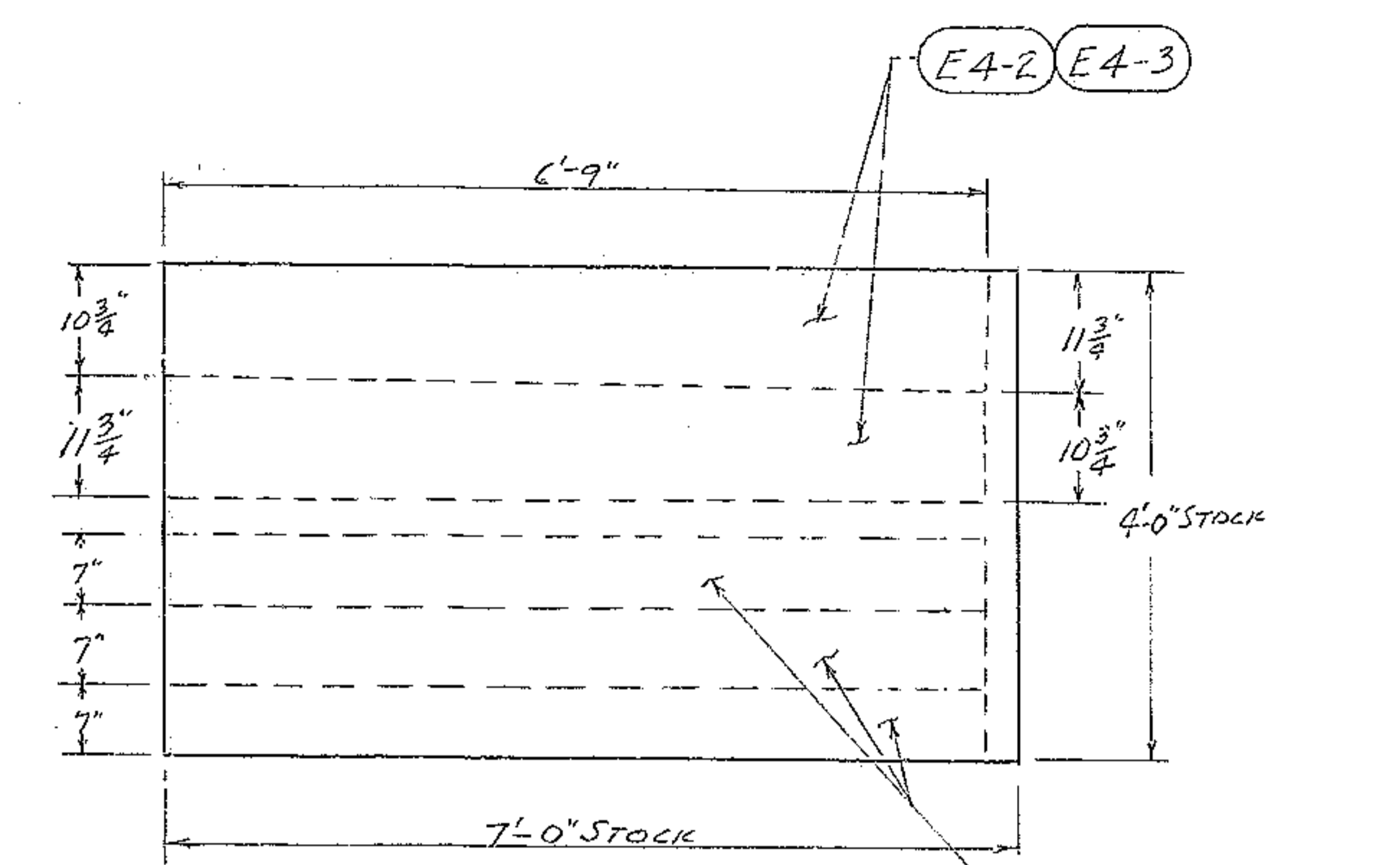
CUTTING LAYOUT SHEET C 1 REQ'D - 3/4" x 1'-0"
