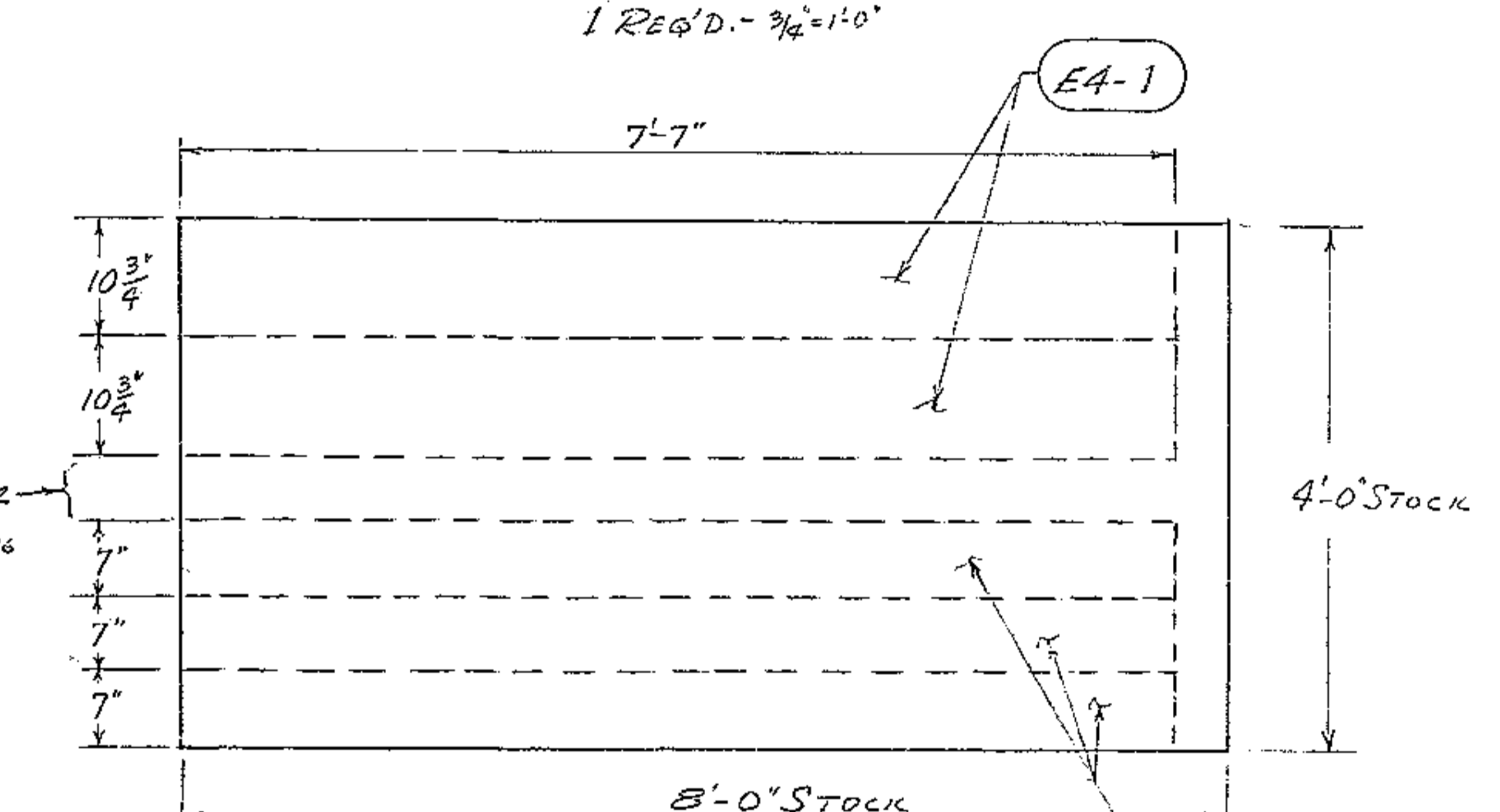
CUTTING LAYOUT SHEET D 1 REQ'D - 3/4" x 1'-0"
