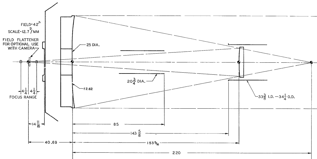
84 INCH TELESCOPE F/7.6 RITCHY CHRÉTIEN FOCUS
